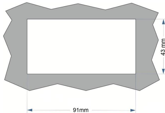
View Dimension
